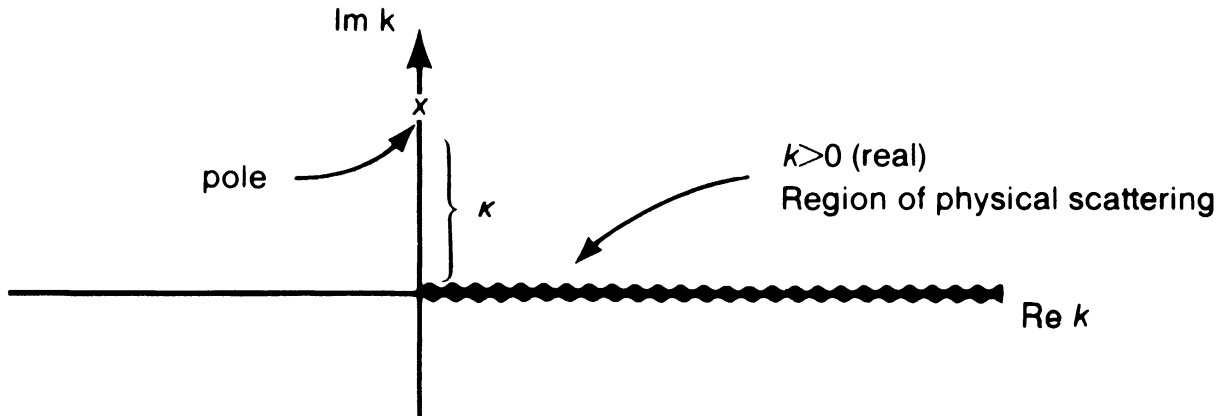
FIGURE 7.10. The complex k -plane with bound-state pole at k = +i\kappa .
