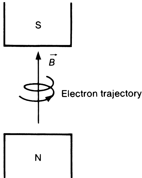
FIGURE 4.10. Electron trajectory between the north and south poles of a magnet.
