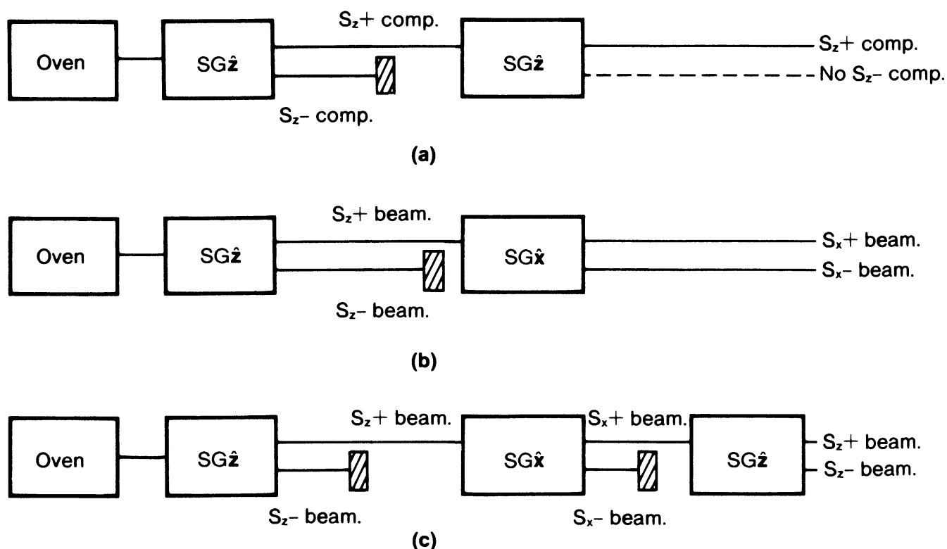
FIGURE 1.3. Sequential Stern-Gerlach experiments.
