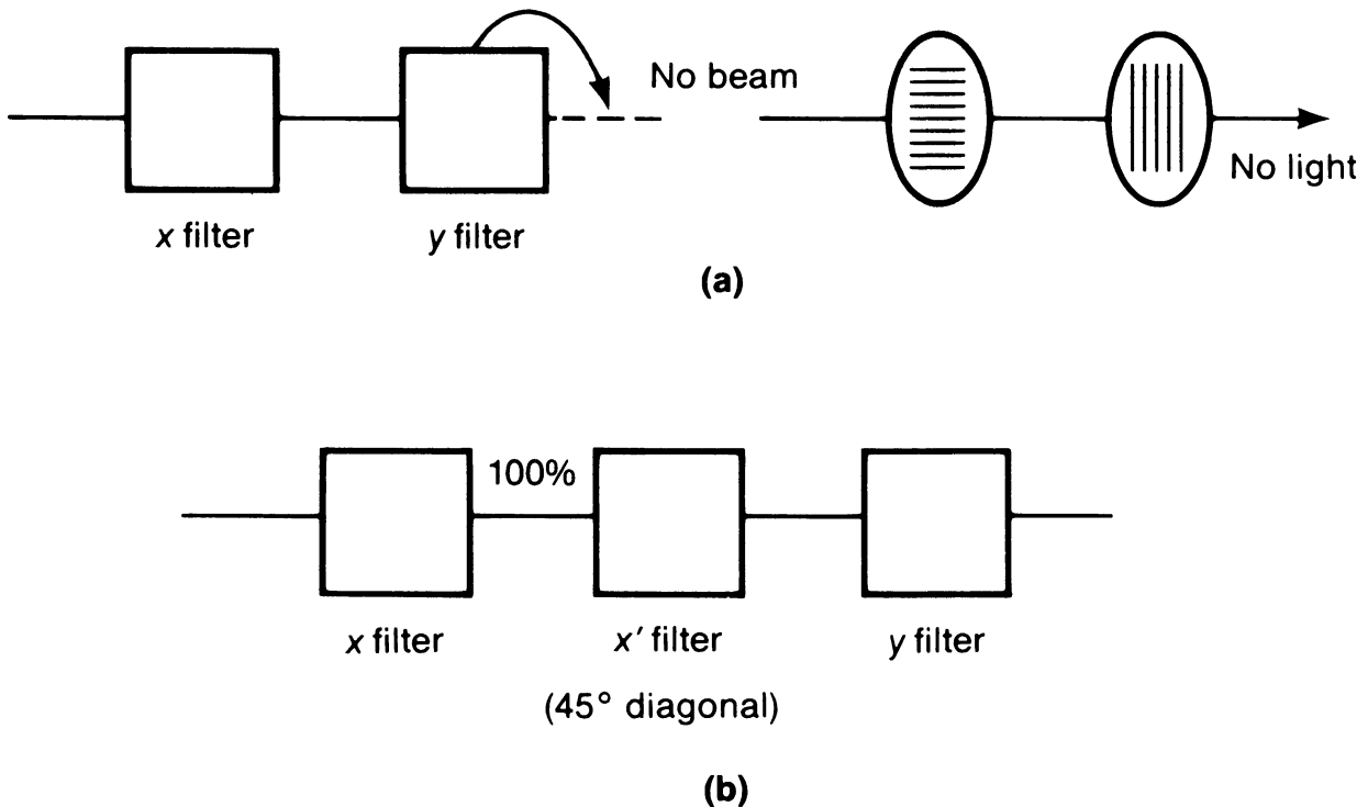
FIGURE 1.4. Light beams subjected to Polaroid filters.
