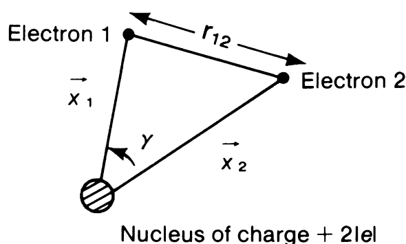
FIGURE 6.3. Schematic diagram of the helium atom.
