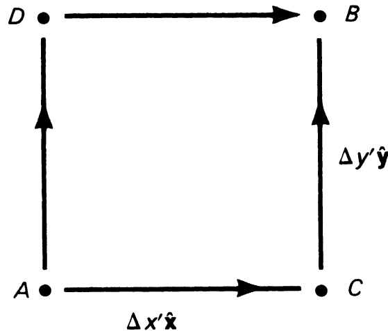
FIGURE 1.8. Successive translations in different directions.
