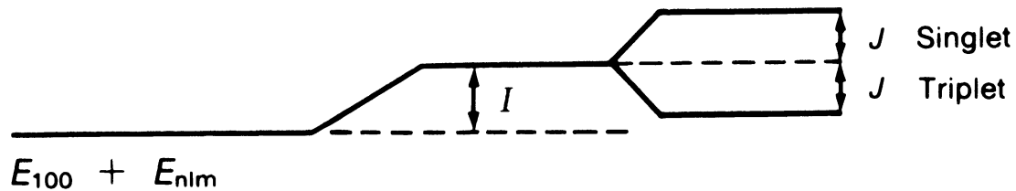
FIGURE 6.4. Schematic diagram for the energy-level splittings of (1s)(nl) for the helium atom.
