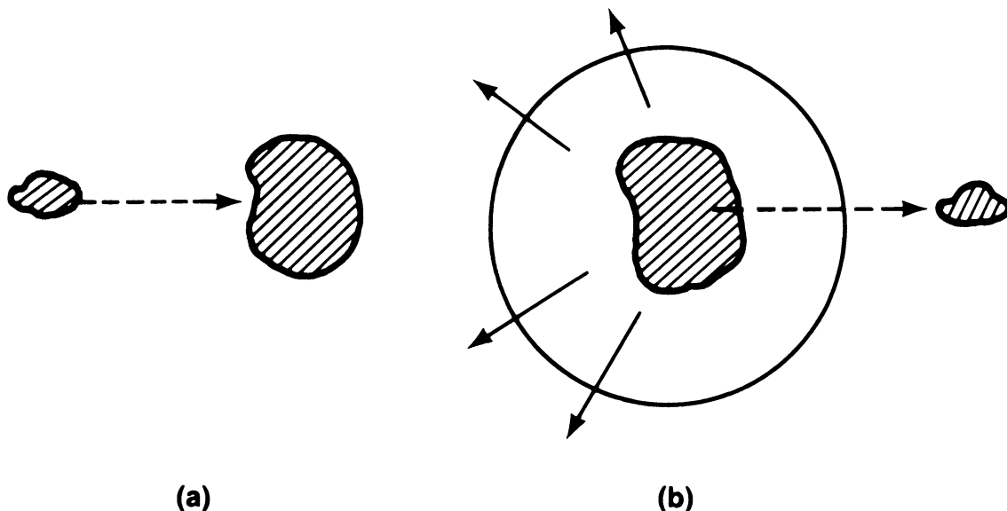
FIGURE 7.2. (a) Incident wave packet approaching scattering center initially. (b) Incident wave packet continuing to move in the original direction plus spherical outgoing wave front (after a long time duration).
