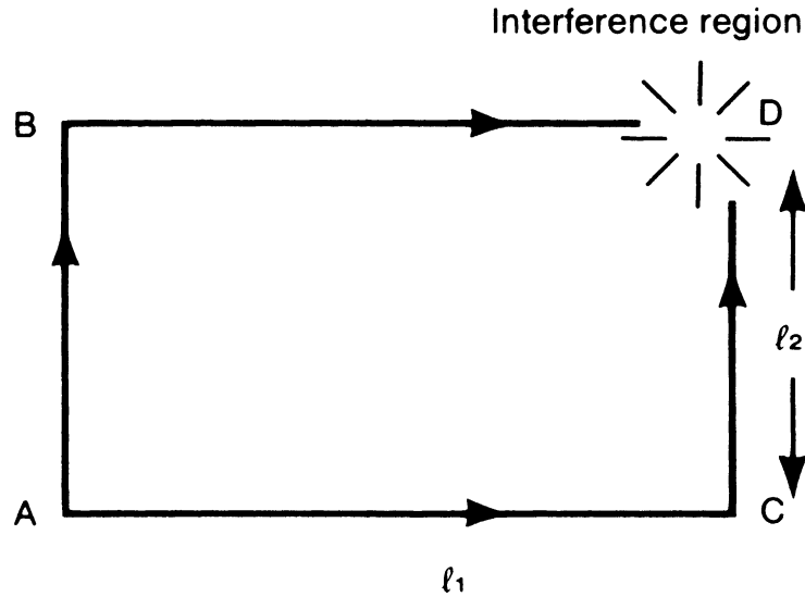
FIGURE 2.5. Experiment to detect gravity-induced quantum interference.
