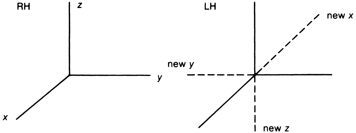
FIGURE 4.1. Right-handed (RH) and left-handed (LH) systems.
