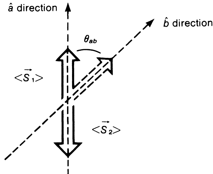
FIGURE 3.9. Evaluation of P(\hat{\mathbf{a}}+; \hat{\mathbf{b}}+) .
