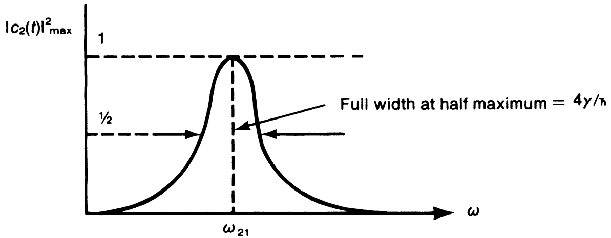
FIGURE 5.5. Graph of |c_2(t)|^2_{\max} as a function of \omega , where \omega = \omega_{21} corresponds to the resonant frequency.
