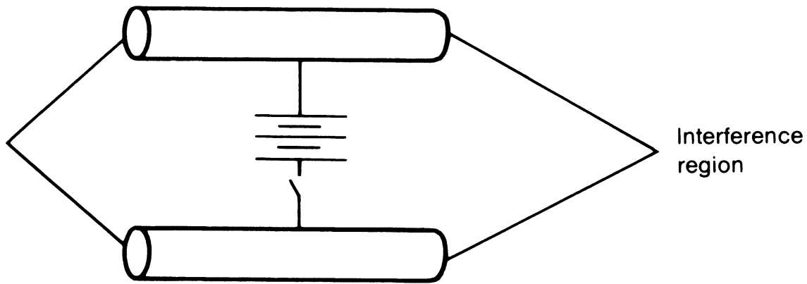
FIGURE 2.4. Quantum-mechanical interference to detect a potential difference.
