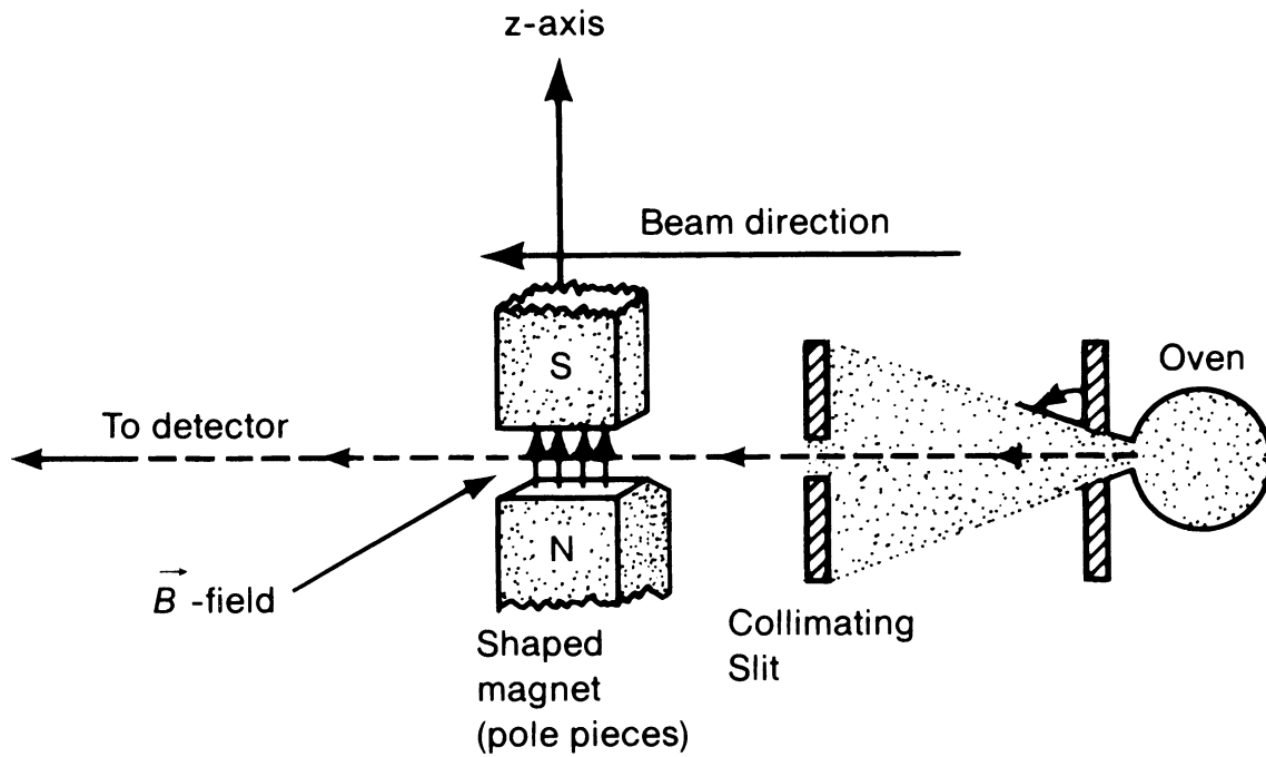
FIGURE 1.1. The Stern-Gerlach experiment.
