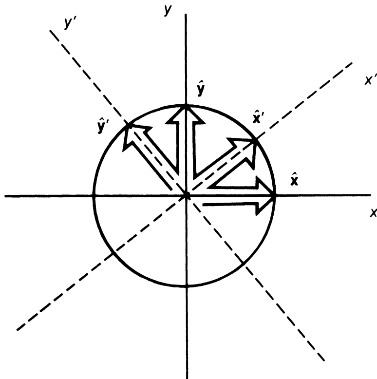
FIGURE 1.5. Orientations of the x' - and y' -axes.
