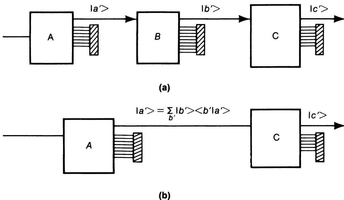
FIGURE 1.7. Sequential selective measurements.
