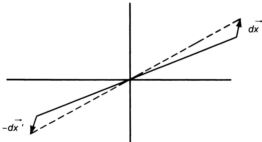
FIGURE 4.2. Translation followed by parity, and vice versa.
