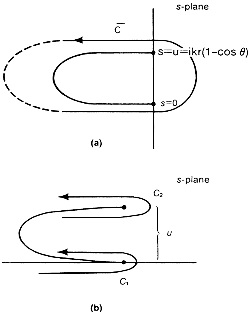
FIGURE C.2. (a) s -plane contour \bar{C} for Equation (C.1.6). (b) Rubber-band distortion of \bar{C} into C_1 plus C_2 .
